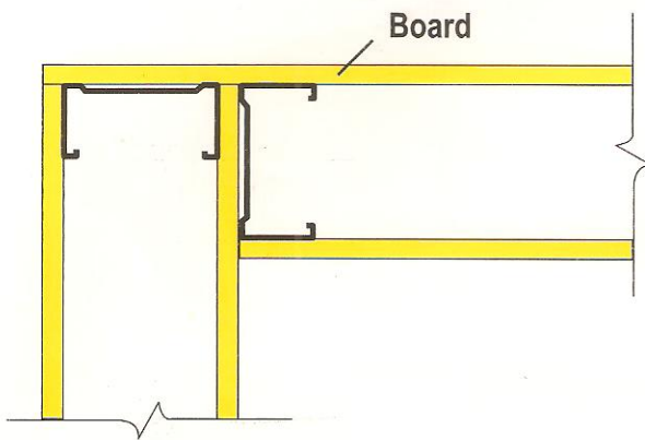
CORNER JOINT
