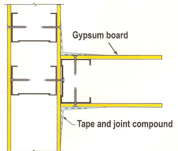
WALL INTERSECTION
