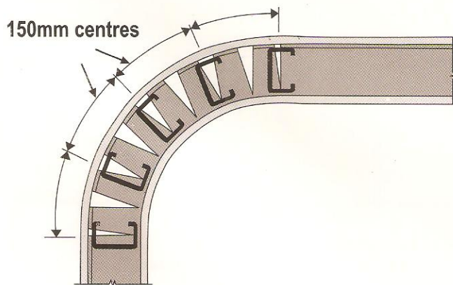
CURVED WALL
