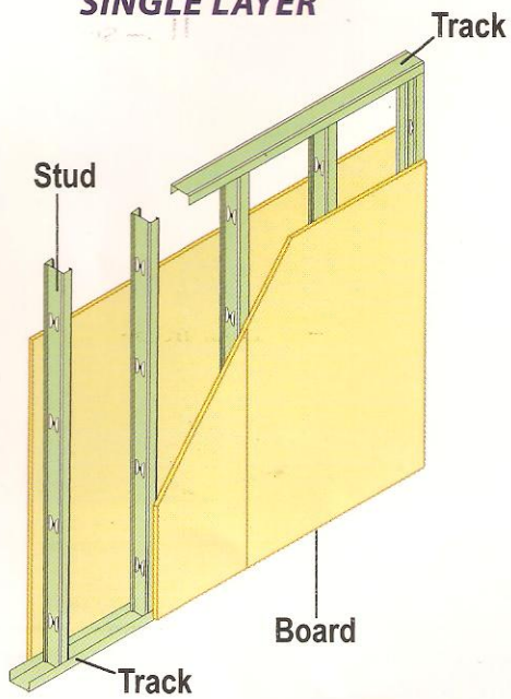
SINGLE LAYER
